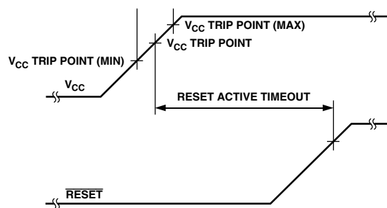
Figure 3. V_{CC} Power-Up Timing Diagram
